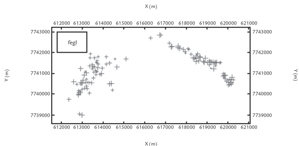
Figure 03 Map of the spatial distribution of selected samples for studies of variability in the mine of João Pereira
