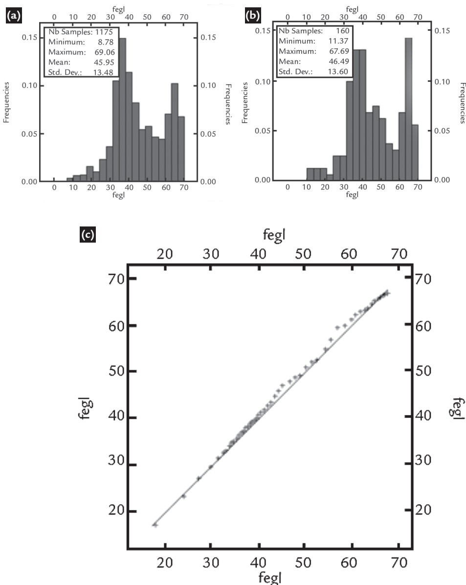
Figure 04 a) histogram of all samples of lithotypes chosen; b) Histogram of selected samples; c) QQ-Plot showing the adhesion between the selected samples and the straight-line identity.
