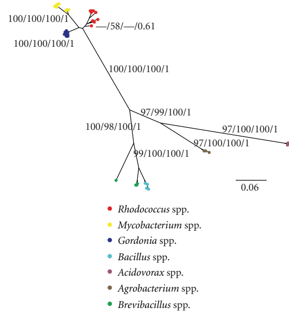
FIGURE 1: Tree obtained by BA analysis from sequences of the 16S gene. The values on the branches represent bootstrap values of NJ, MV, and MP and posterior probability of the BA analysis.
